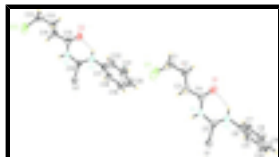
Fig. 1. The molecular structure of (I), with displacement ellipsoids are drawn at the 50% probability level. the dashed line denote the intramolecular hydrogen bonds.
