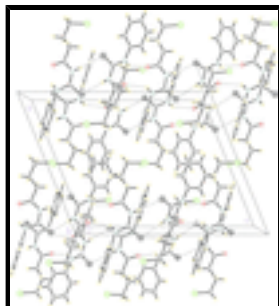
Fig. 2. The molecular packing of (I) viewed down the b-axis. The dashed line denote the intermolecular hydrogen bonds.
